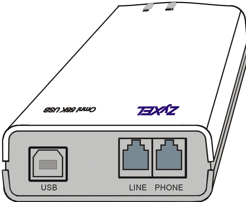
Figure 1. Back Panel
