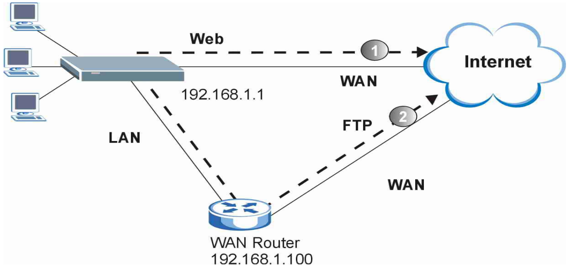
Figure 41-6 Example of IP Policy Routing
