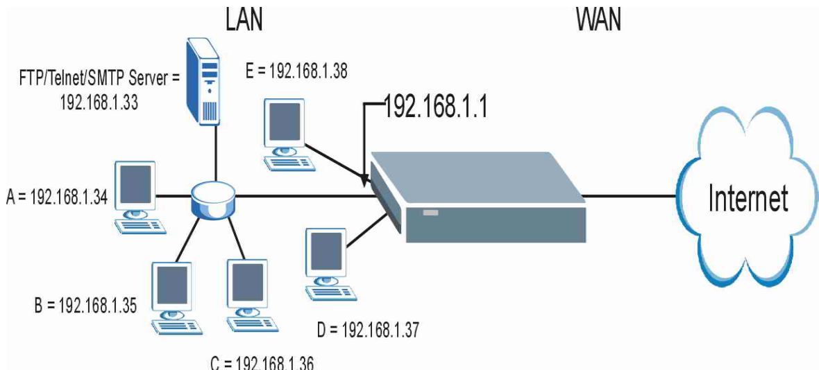
Figure 32-10 Multiple Servers Behind NAT Example
