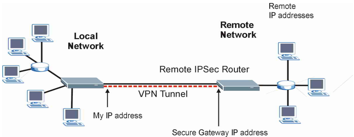
Figure 17-1 IPsec Summary Fields
