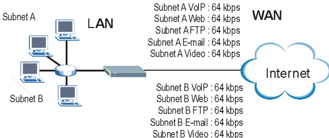
Figure 21-3 Application and Subnet-based Bandwidth Management Example
