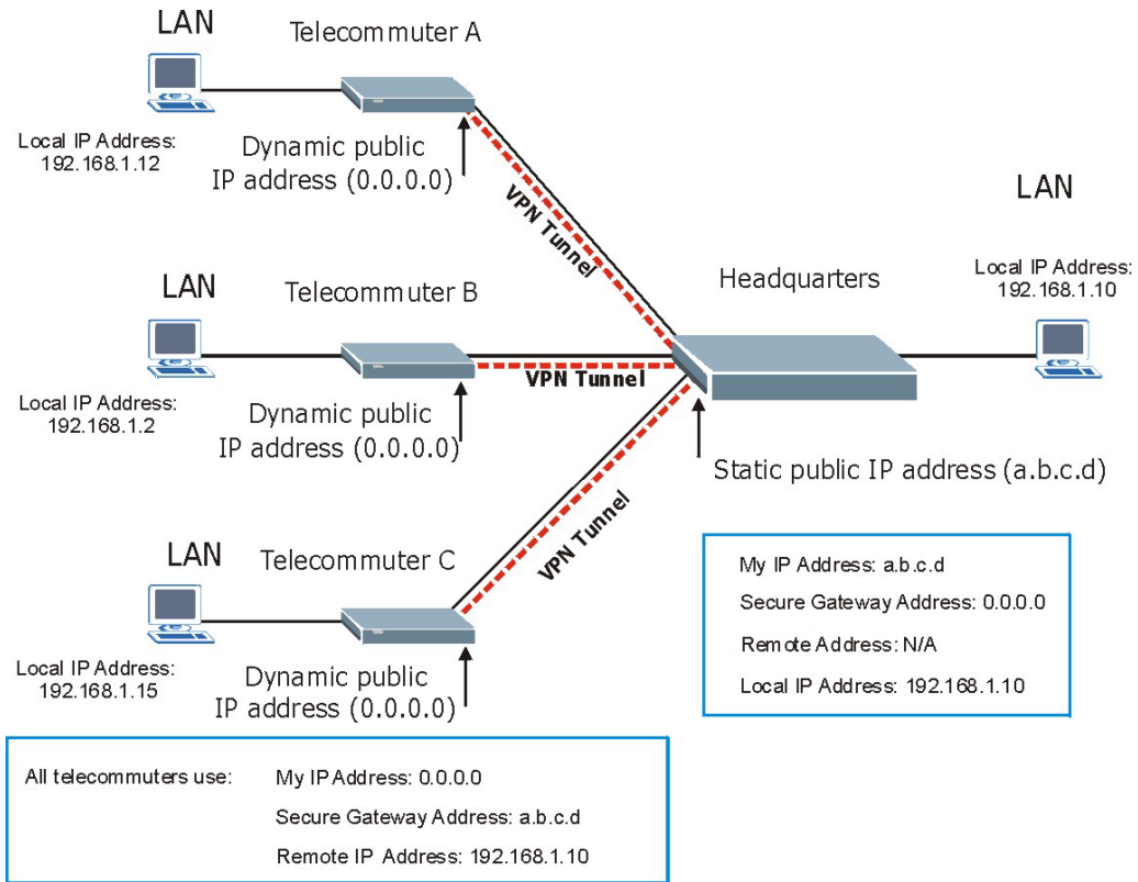
Figure 17-9 Telecommuters Sharing One VPN Rule Example
