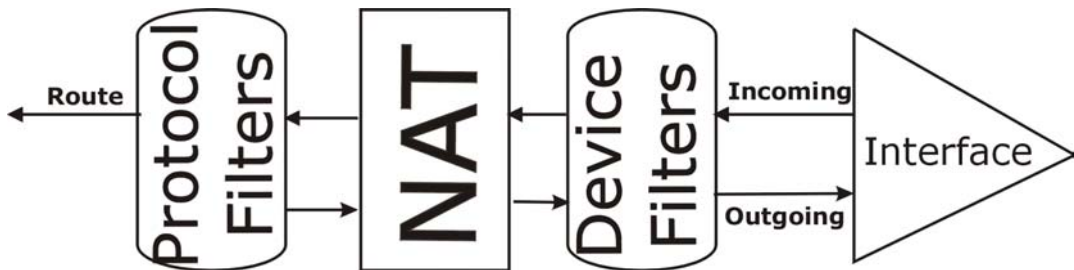
Figure 34-13 Protocol and Device Filter Sets
