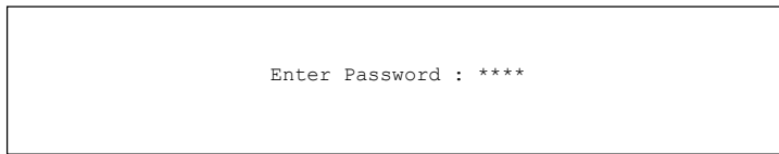
Figure 23-1 Login Screen
