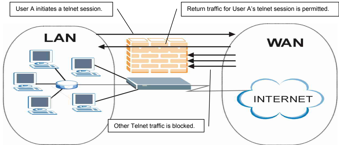
Figure 11-5 Stateful Inspection
