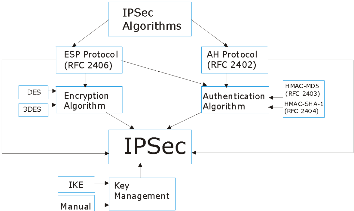
Figure 16-2 IPsec Architecture
