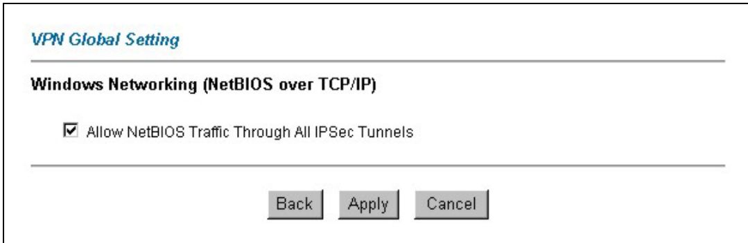
Figure 17-8 Global Setting
