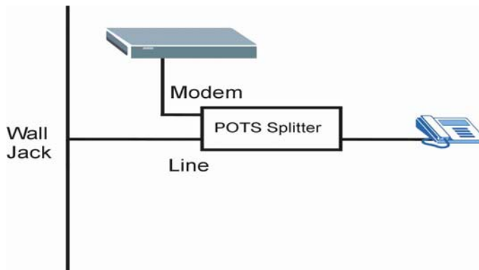
Diagram J-1 Connecting a POTS Splitter
