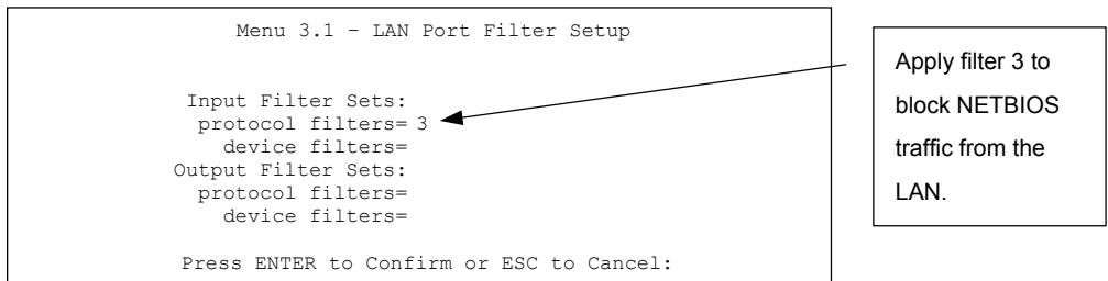
Figure 34-17 Filtering Ethernet Traffic
