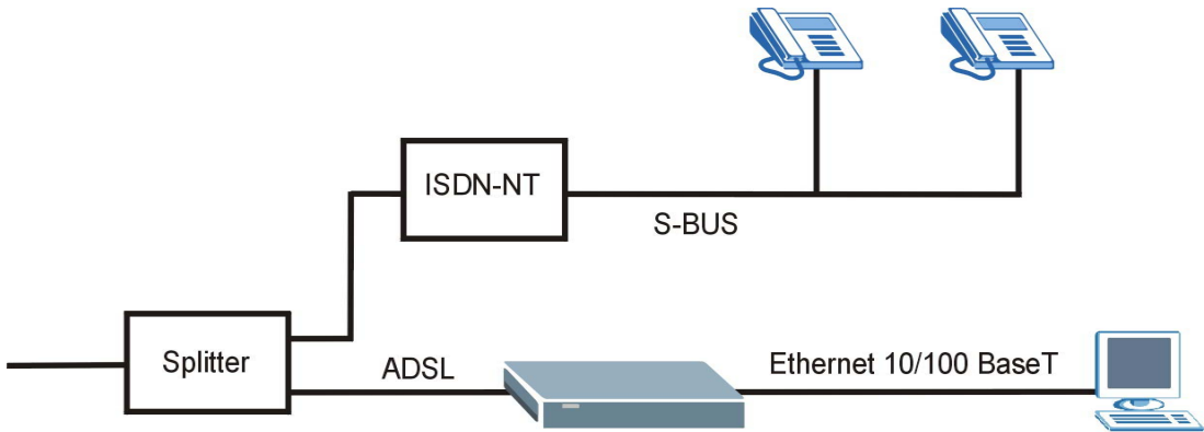
Diagram J-3 Prestige with ISDN
