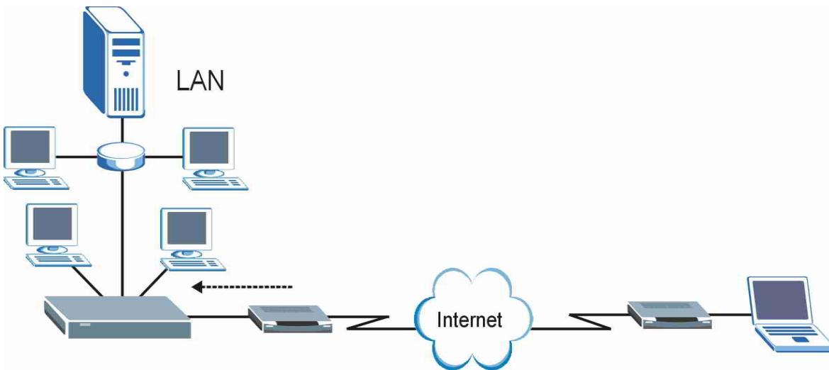
Figure 18-1 Telnet Configuration on a TCP/IP Network
