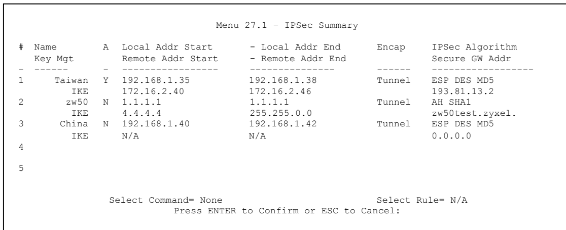
Figure 43-3 Menu 27.1 IPSec Summary
