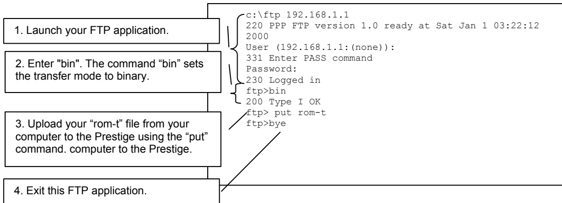
Figure 45-5 Internal SPTGEN FTP Upload Example
