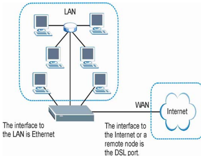
Figure 5-1 LAN and WAN IP Addresses
