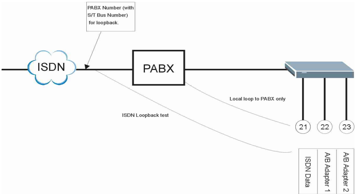
Figure 25-4 Router Behind a PABX
