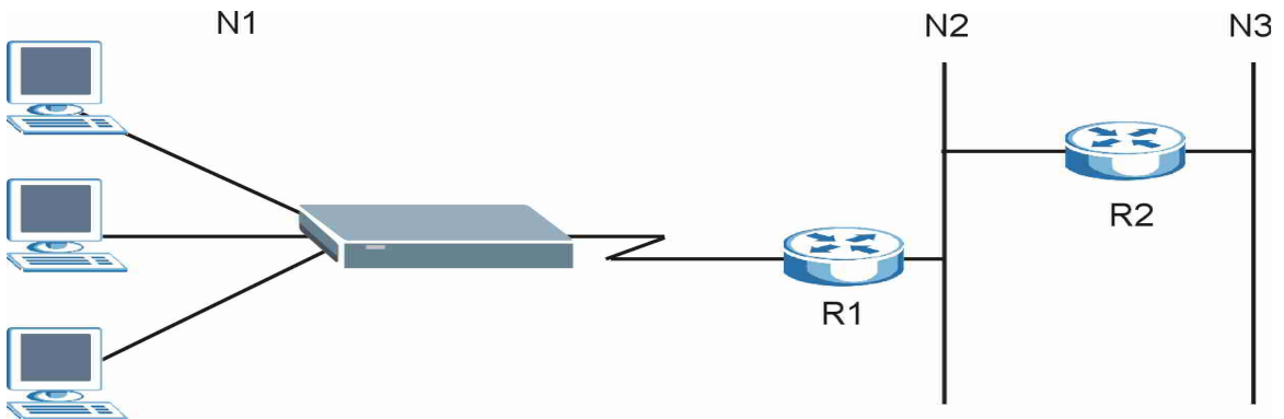
Figure 30-1 Sample Static Routing Topology
