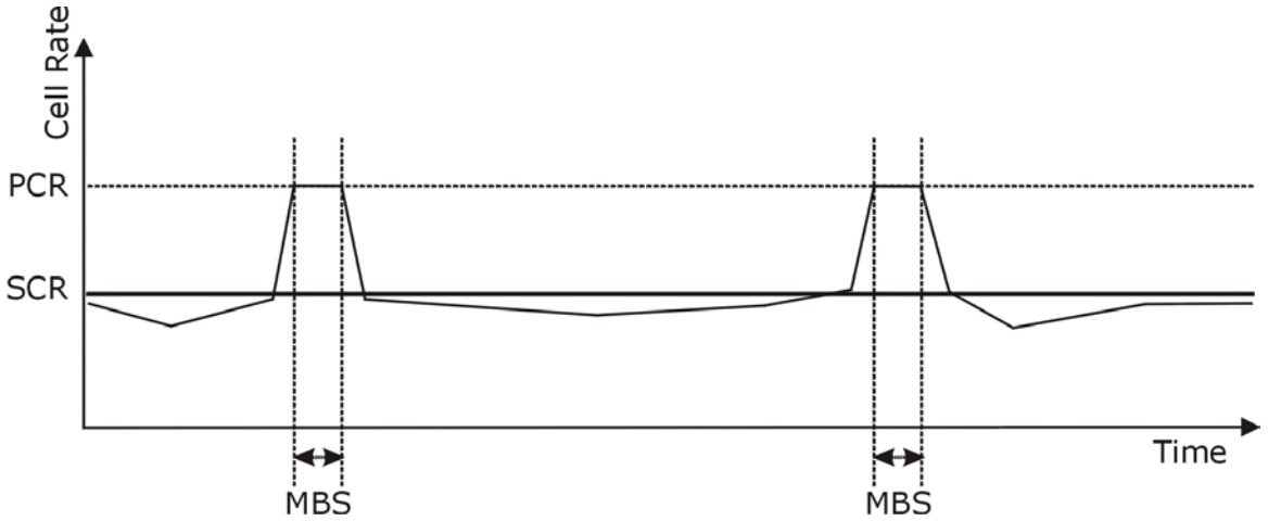
Figure 7-1 Example of Traffic Shaping
