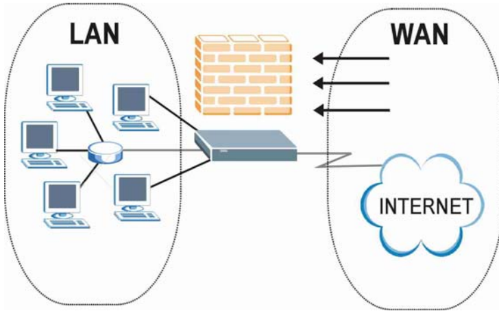
Figure 1-2 Firewall Application
