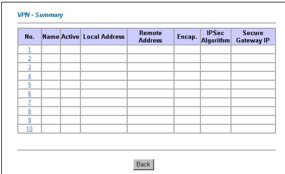
Figure 17-2 VPN Summary
