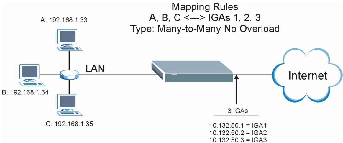
Figure 32-19 NAT Example 4
