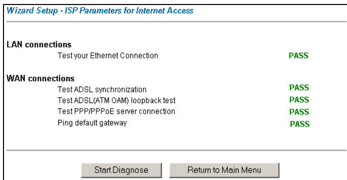
Figure 3-8 Wizard Screen 4
