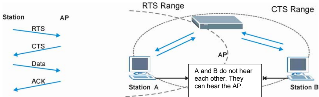
Figure 6-1 RTS Threshold
