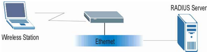
Figure 6-5 EAP Authentication
