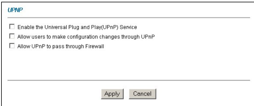
Figure 19-1 Configuring UPnP
