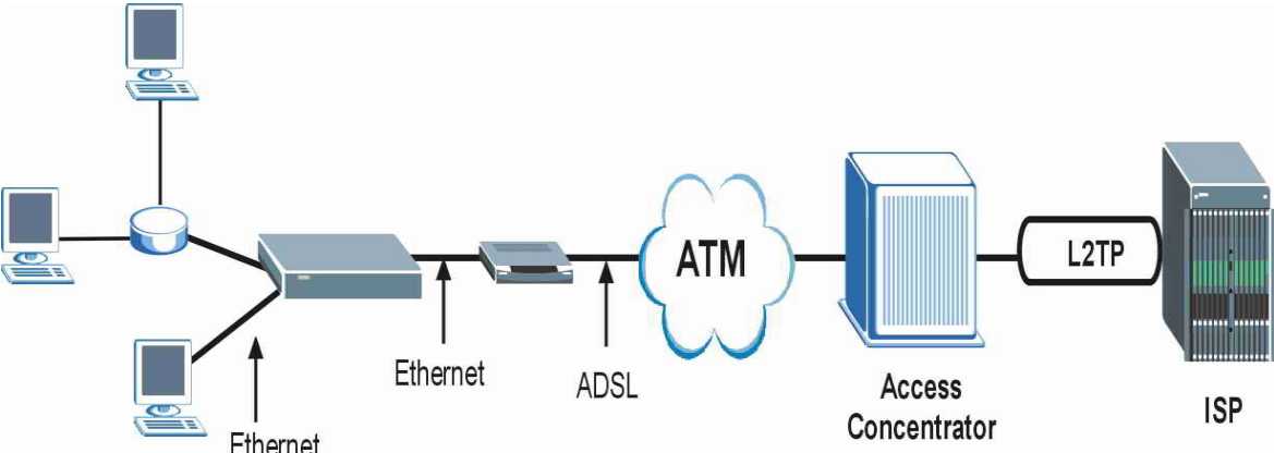
Diagram E-2 Prestige as a PPPoE Client
