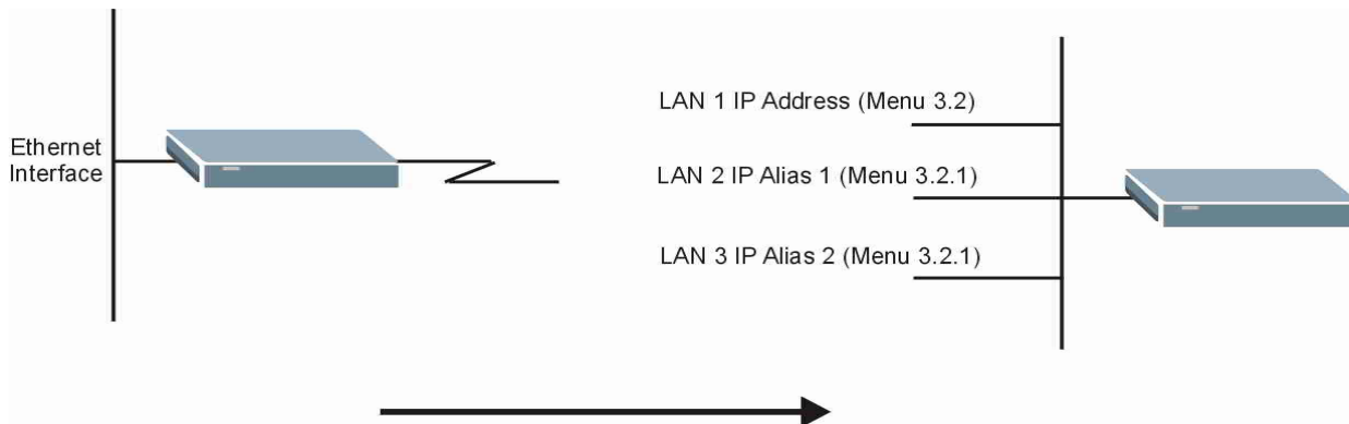
Figure 28-1 Physical Network
