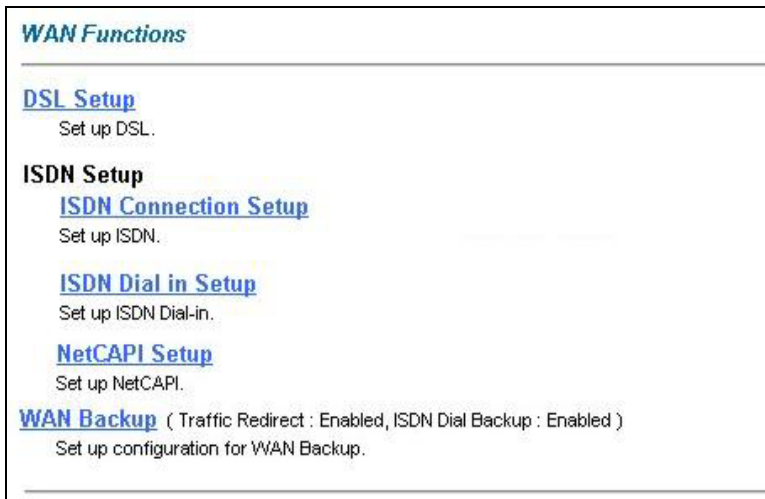
Figure 7-2 WAN Functions
