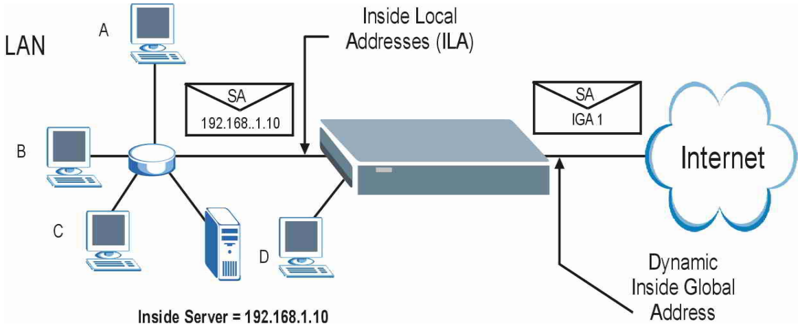
Figure 32-13 NAT Example 2
