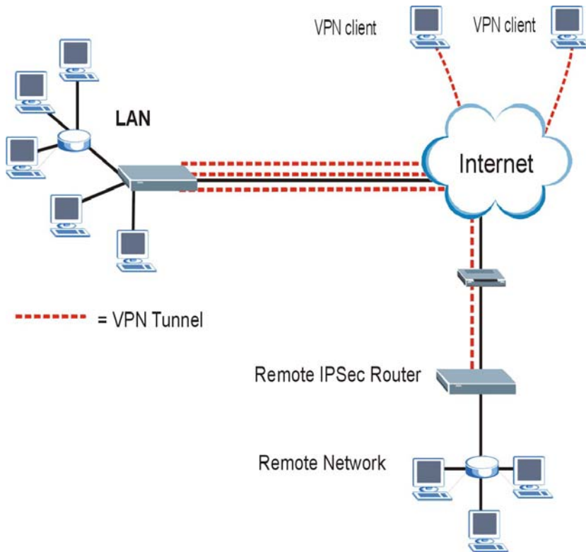
Figure 1-3 VPN Application
