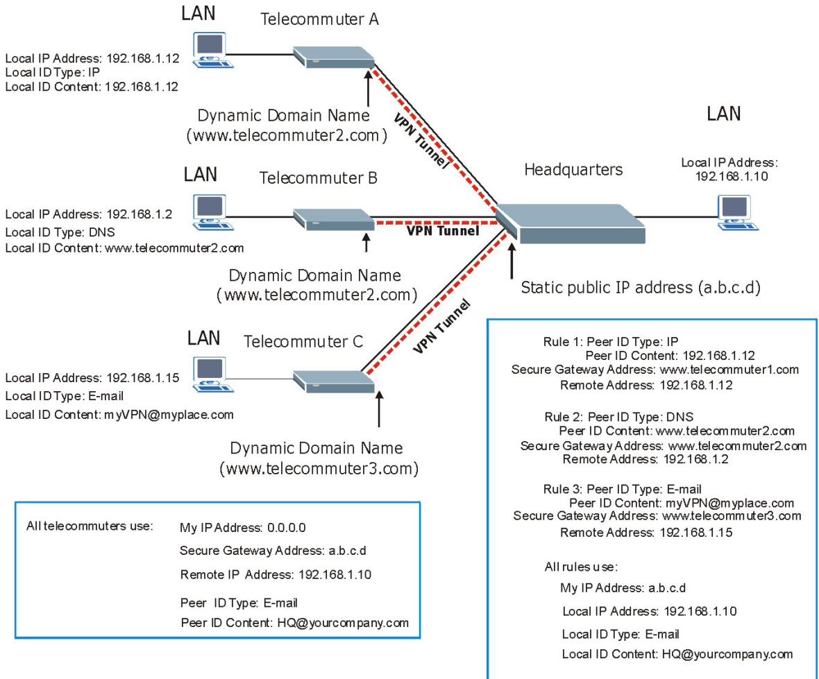
Figure 17-10 Telecommuters Using Unique VPN Rules Example
