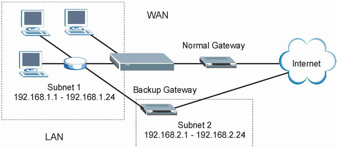
Figure 7-10 Traffic Redirect LAN Setup
