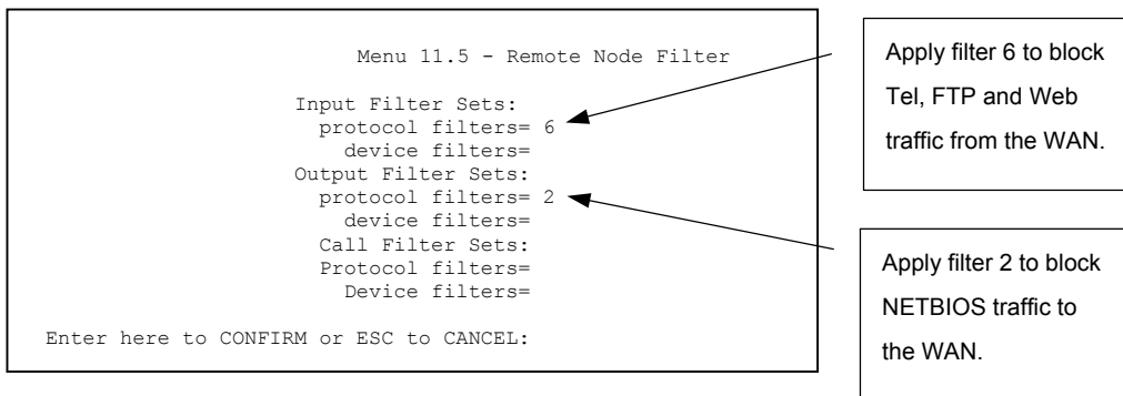
Figure 34-18 Filtering Remote Node Traffic
