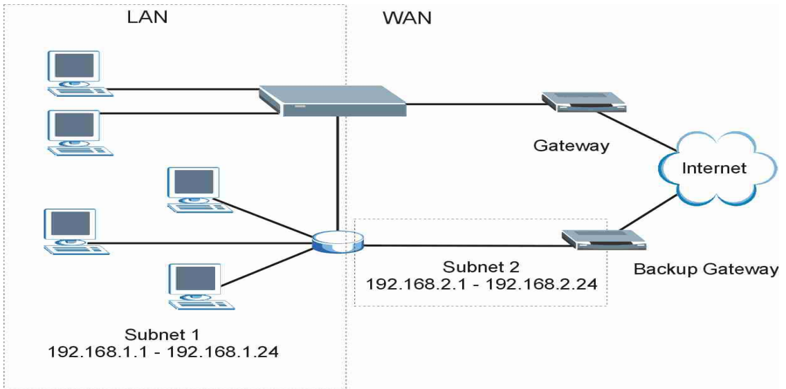
Figure 7-9 Traffic Redirect WAN Setup
