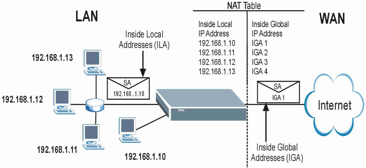
Figure 8-1 How NAT Works
