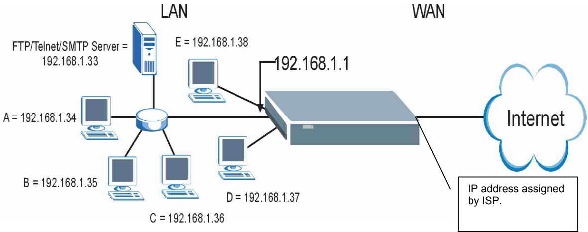
Figure 8-3 Multiple Servers Behind NAT Example
