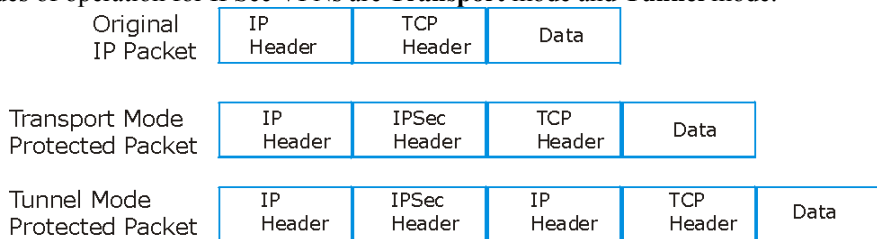
Figure 16-3 Transport and Tunnel Mode IPSec Encapsulation
