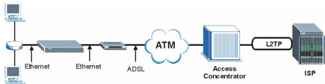
Figure 20 Prestige as a PPPoE Client
