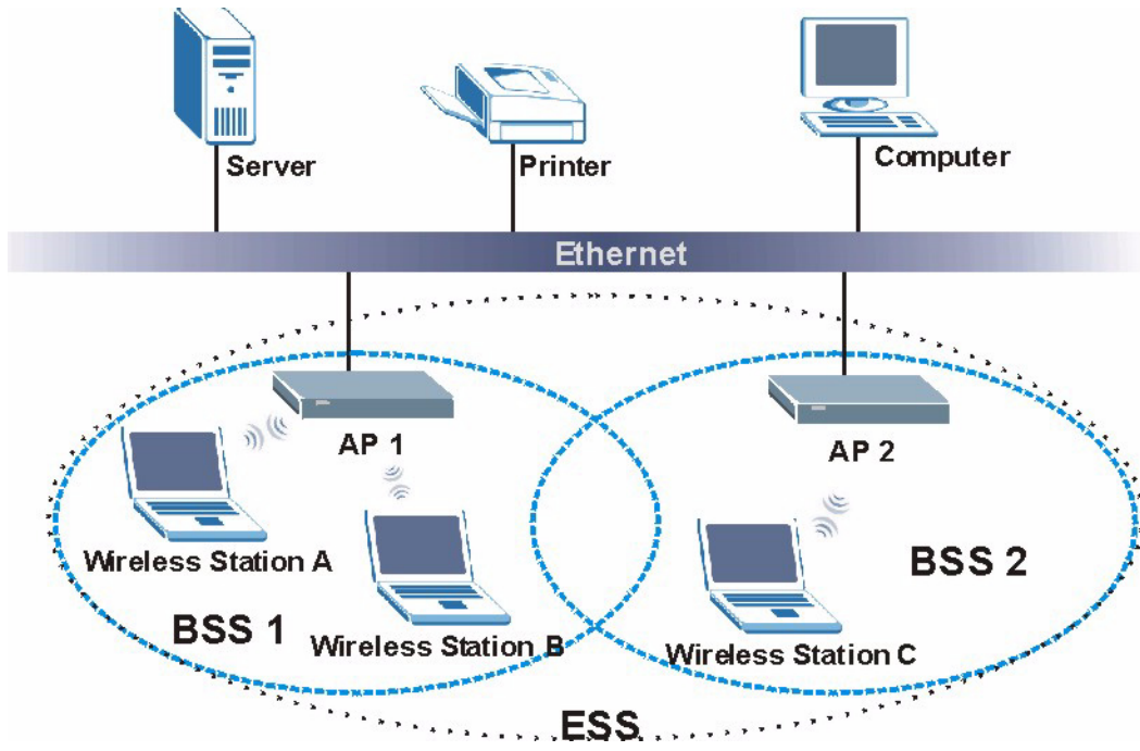
Figure 23 ESS Provides Campus-Wide Coverage
