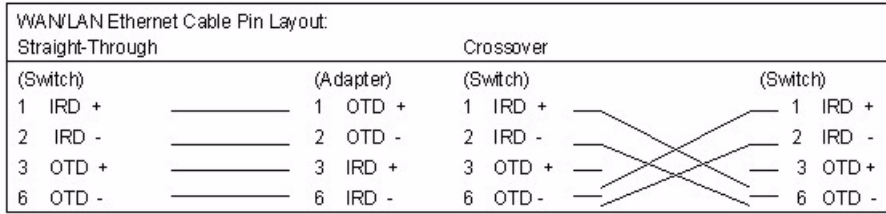
Figure 2 Ethernet Cable Pin Assignments
