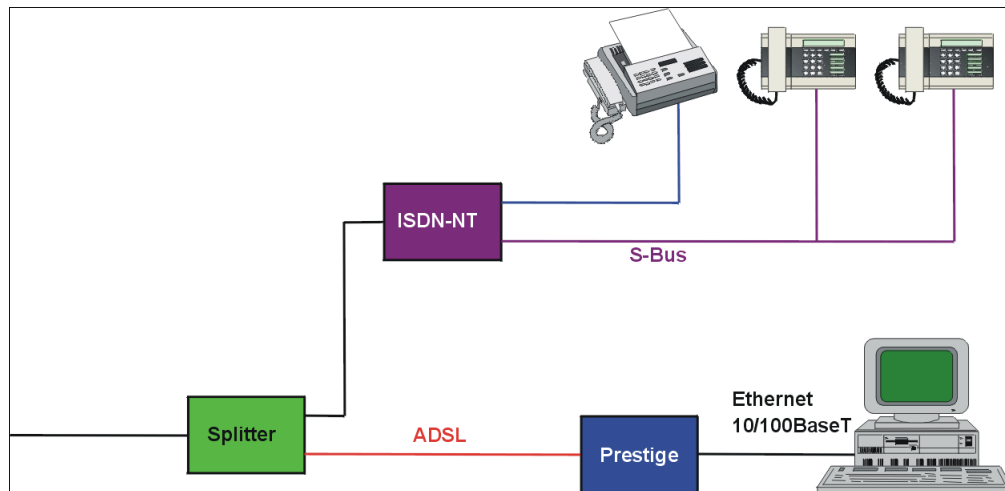
Figure 5 Prestige with ISDN
