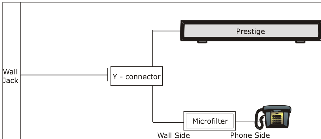
Figure 4 Connecting a Microfilter
