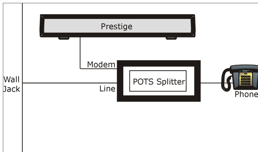
Figure 3 Connecting a POTS Splitter
