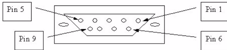
Figure 1 Console/Dial Backup Port Pin Layout
