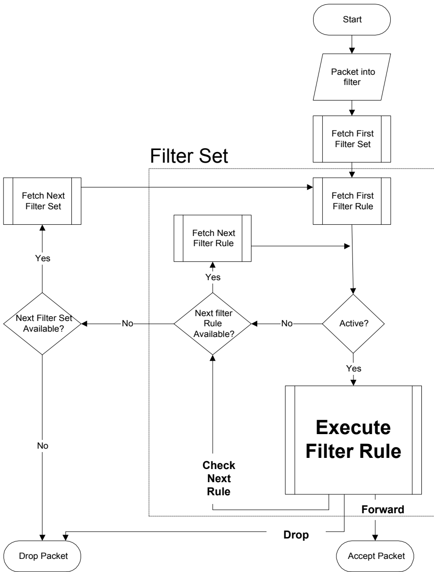
Figure 30-2 Filter Rule Process
