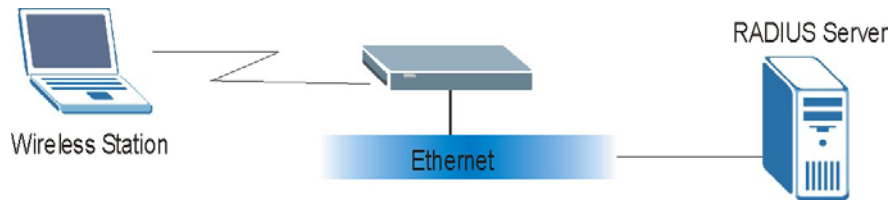
Figure 7-5 EAP Authentication
