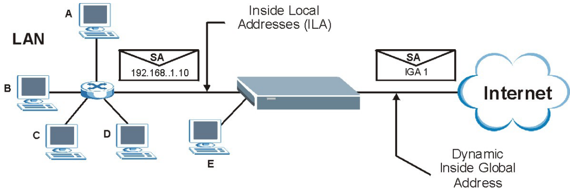
Figure 28-10 NAT Example 1
