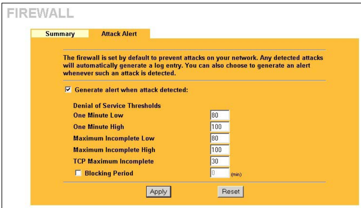
Figure 11-12 Attack Alert
