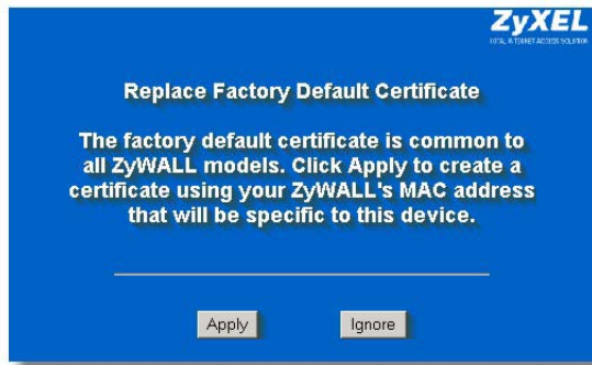
Figure 17-8 Replace Certificate
