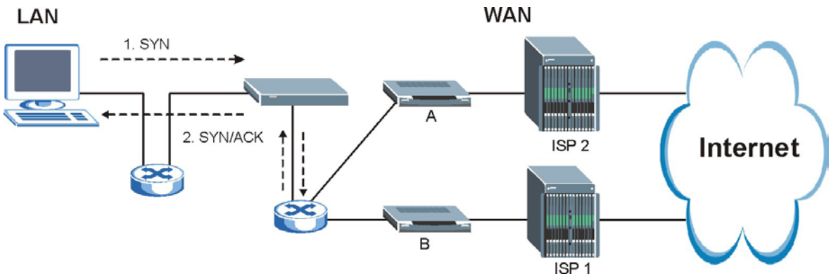
Diagram 4 Gateways on the WAN Side
