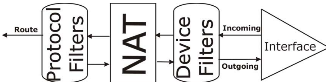
Figure 30-11 Protocol and Device Filter Sets
