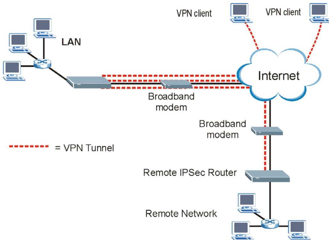
Figure 1-2 Secure Internet Access and VPN Application
