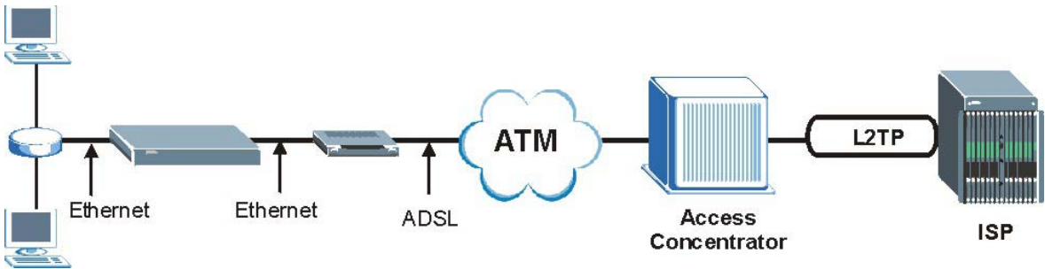
Diagram G-2 ZyWALL as a PPPoE Client
