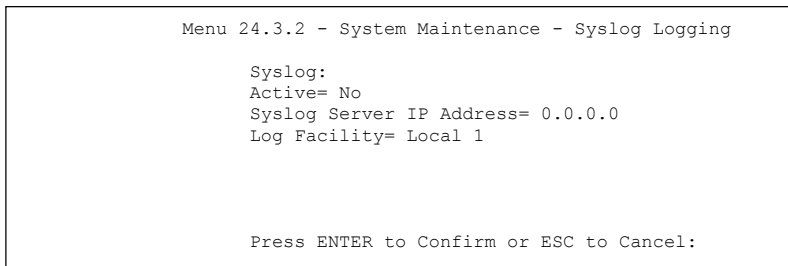
Figure 32-7 Menu 24.3.2: System Maintenance: UNIX Syslog
