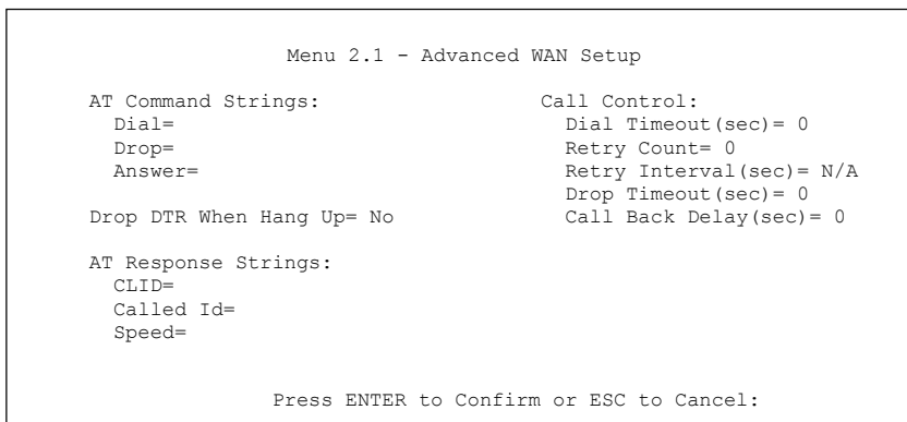
Figure 23-3 Menu 2.1 Advanced WAN Setup
