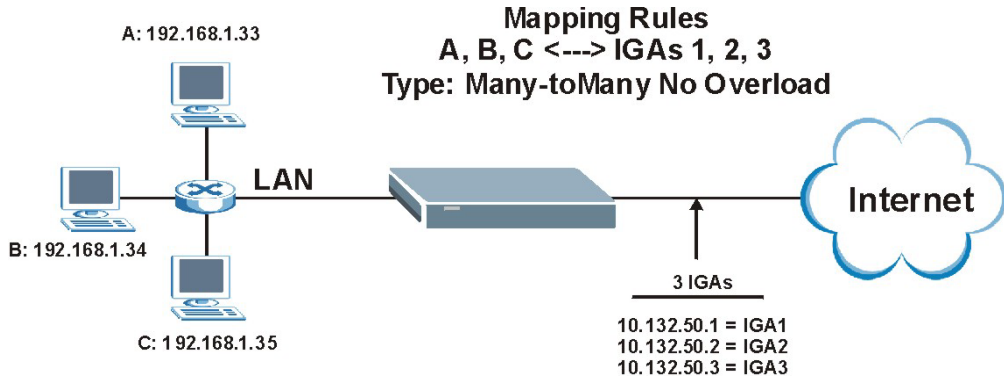
Figure 28-19 NAT Example 4
