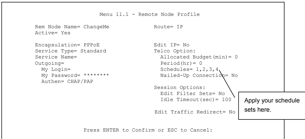
Figure 36-3 Applying Schedule Set(s) to a Remote Node (PPPoE)
