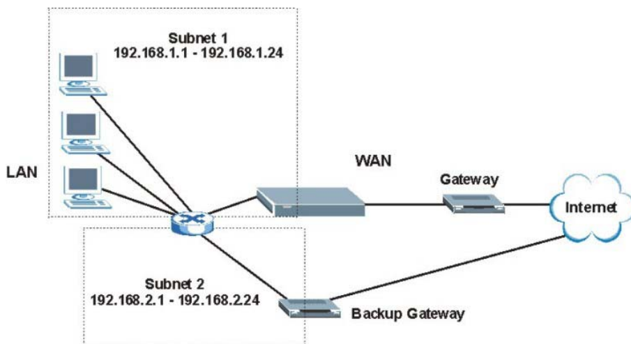
Figure 6-8 Traffic Redirect LAN Setup
