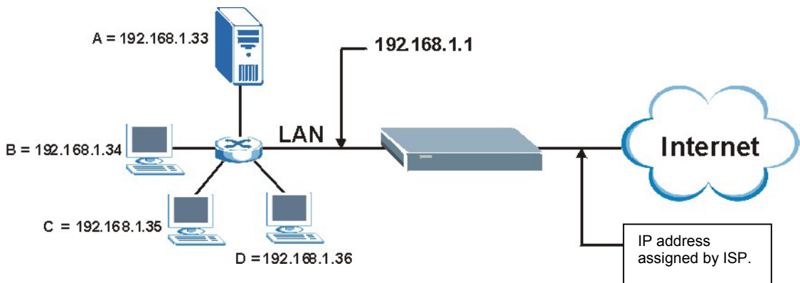
Figure 8-3 Multiple Servers Behind NAT Example
