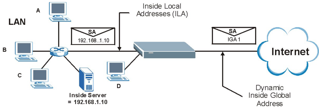
Figure 28-12 NAT Example 2
