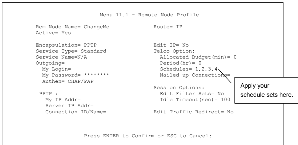
Figure 36-4 Applying Schedule Set(s) to a Remote Node (PPTP)
