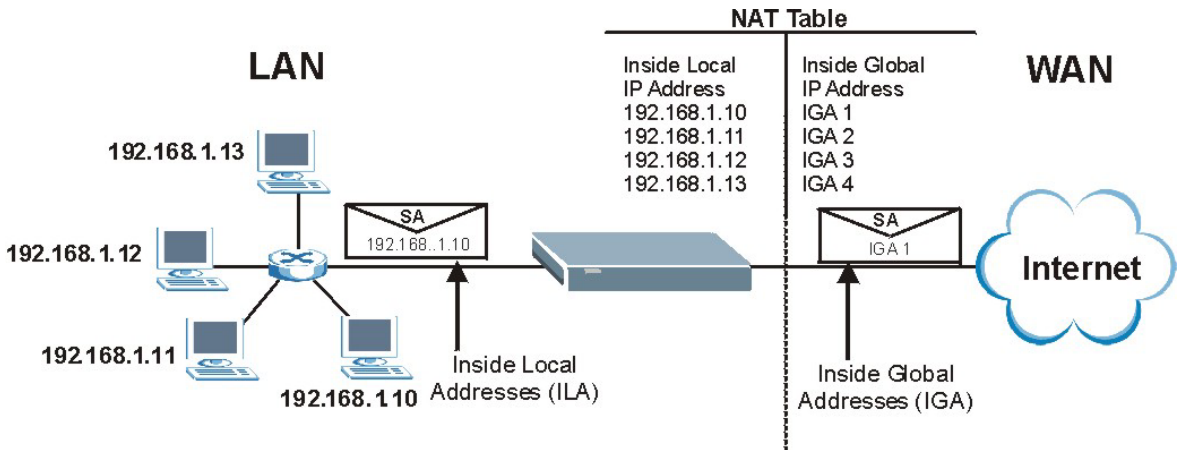
Figure 8-1 How NAT Works
