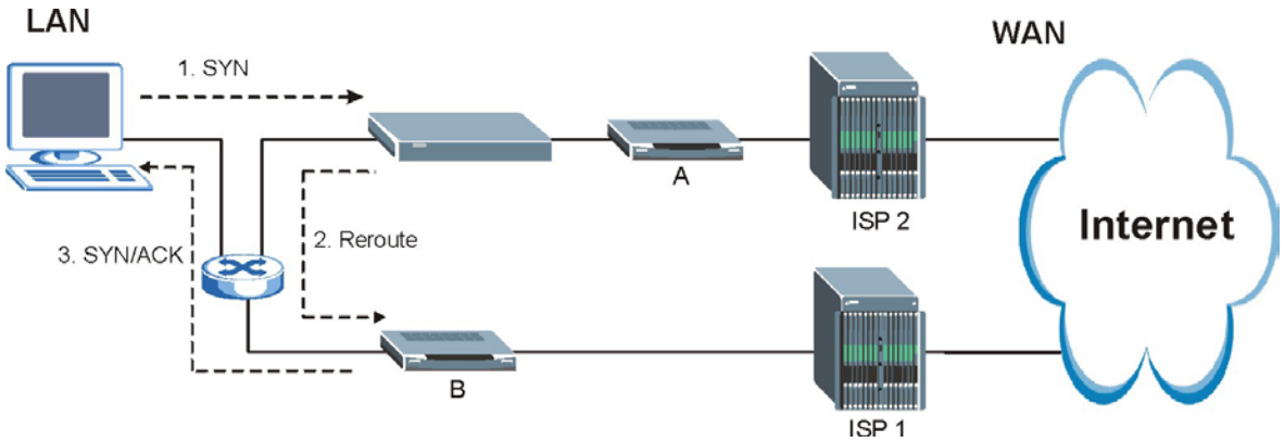
Diagram 2 “Triangle Route” Problem
