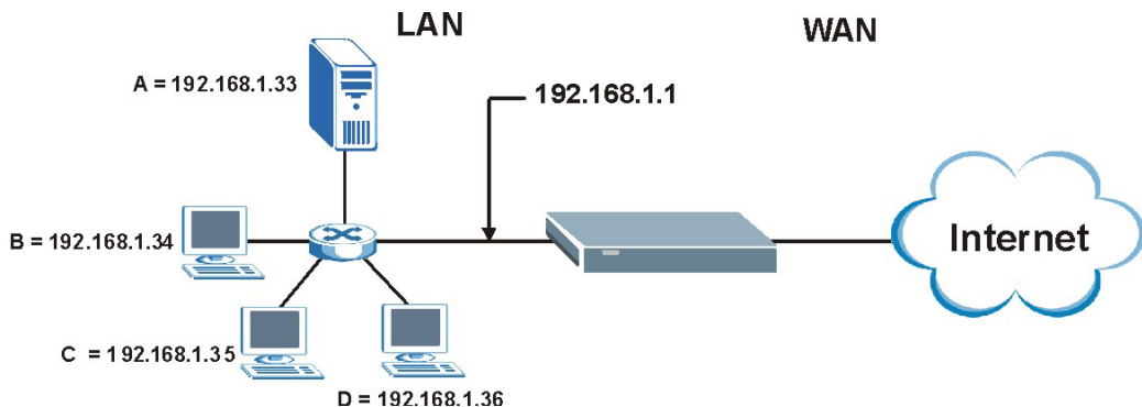
Figure 28-9 Multiple Servers Behind NAT Example
