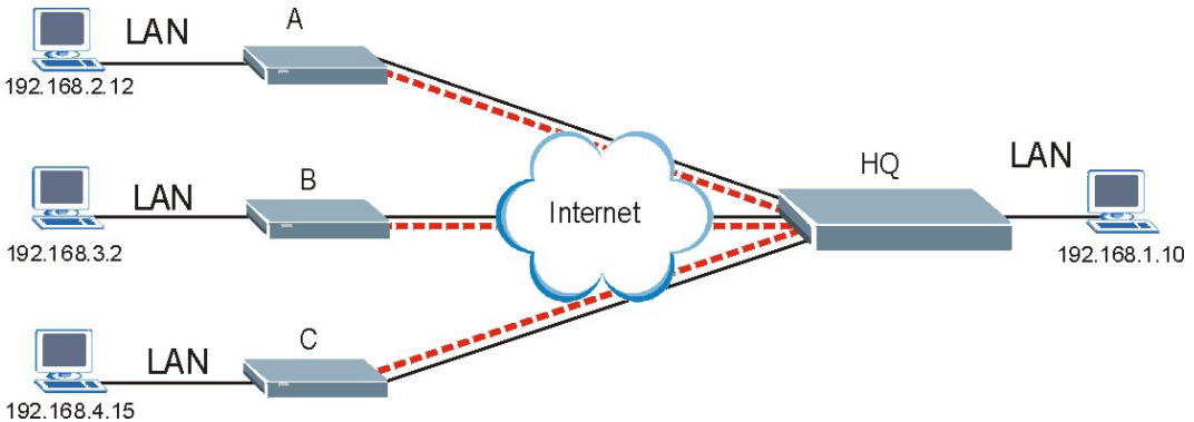
Figure 14-14 Telecommuters Using Unique VPN Rules Example
