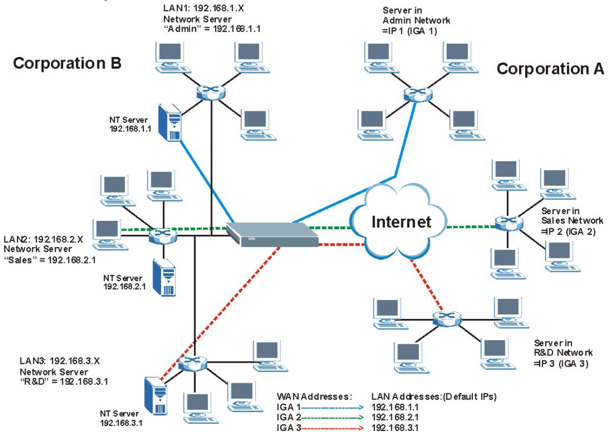
Figure 8-2 NAT Application With IP Alias
