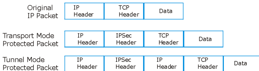
Figure 13-3 Transport and Tunnel Mode IPSec Encapsulation
