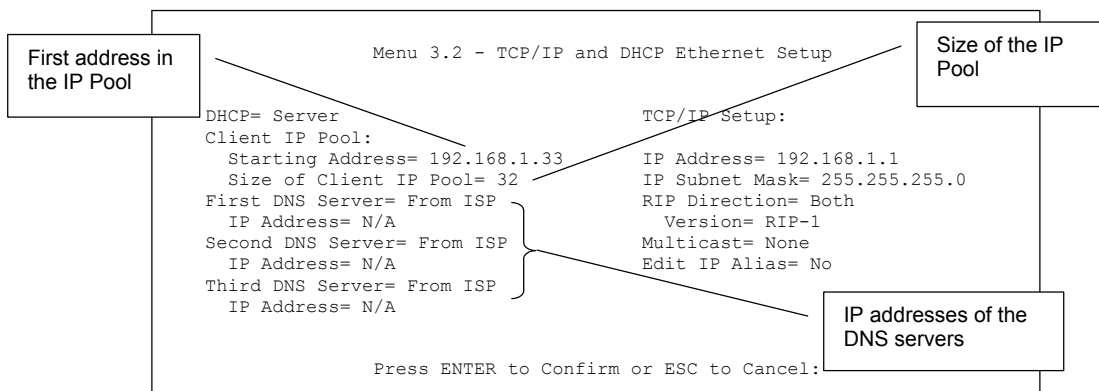
Figure 24-4 Menu 3.2: TCP/IP and DHCP Ethernet Setup
