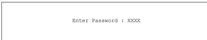
Figure 21-2 Password Screen
