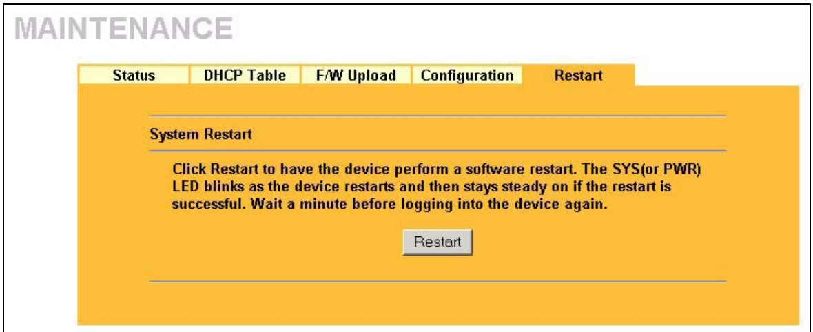
Figure 20-14 Restart Screen
