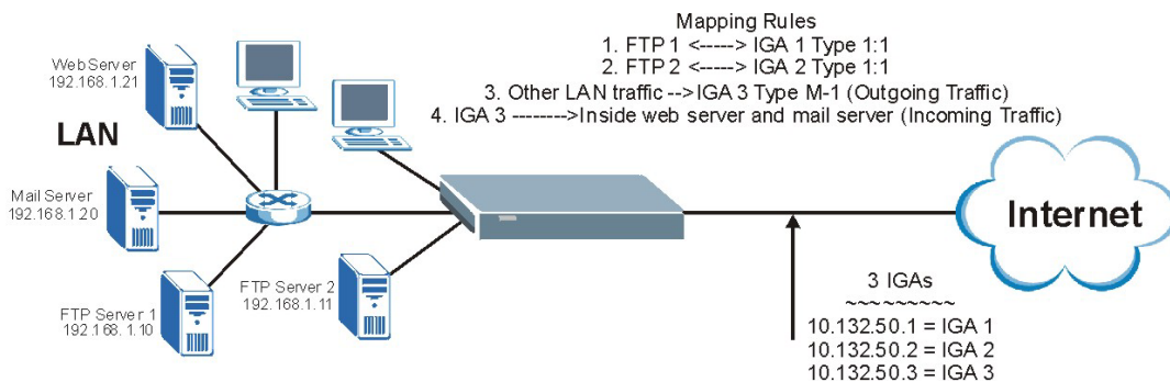
Figure 28-14 NAT Example 3
