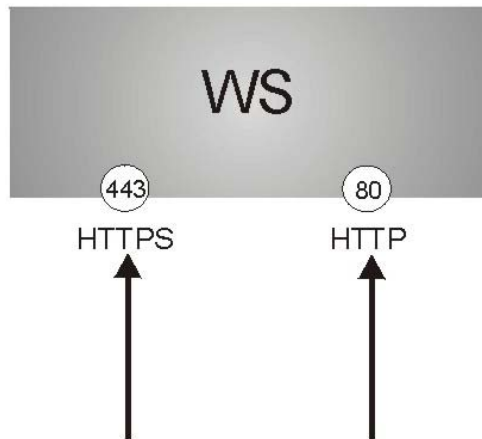
Figure 17-1 HTTPS Implementation
