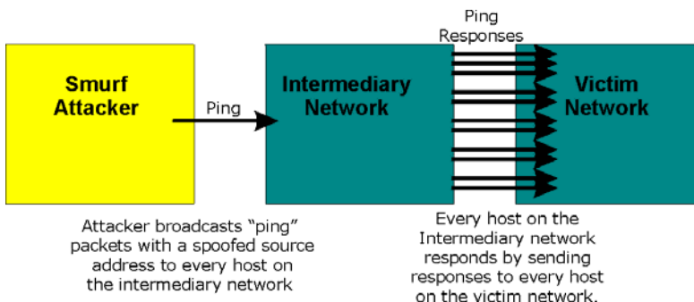
Figure 10-4 Smurf Attack
