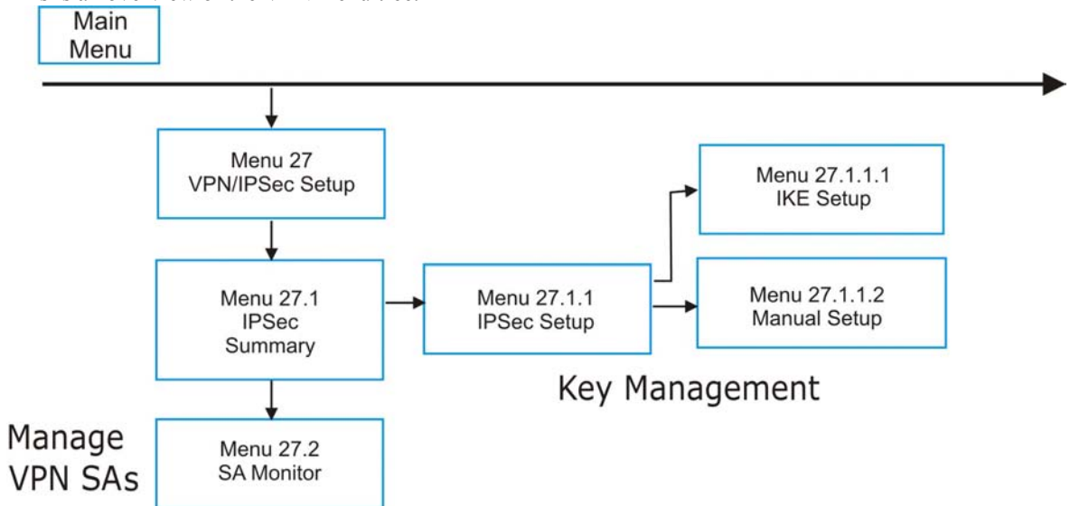
Figure 37-1 VPN SMT Menu Tree
