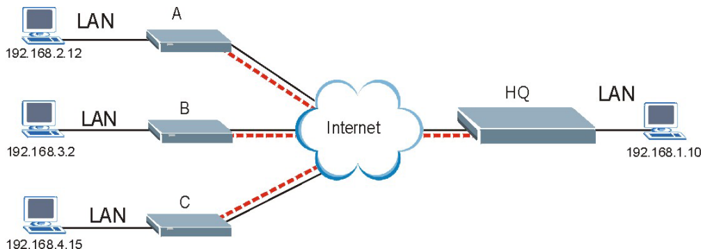
Figure 14-13 Telecommuters Sharing One VPN Rule Example
