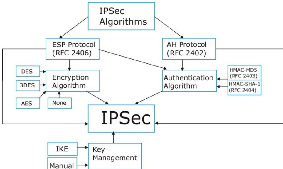
Figure 13-2 IPsec Architecture
