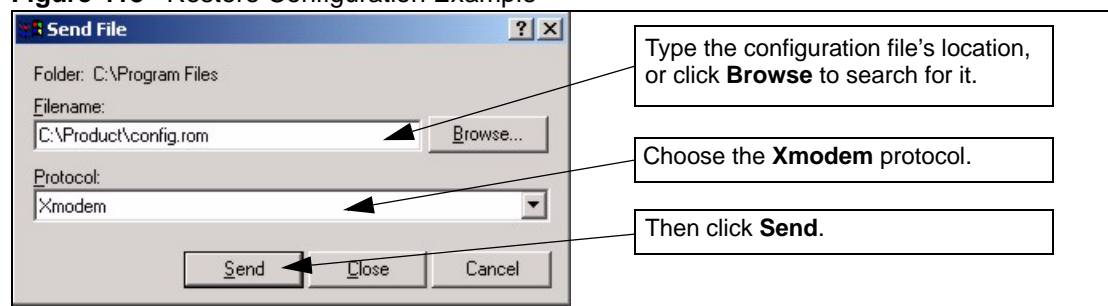
Figure 418 Restore Configuration Example
