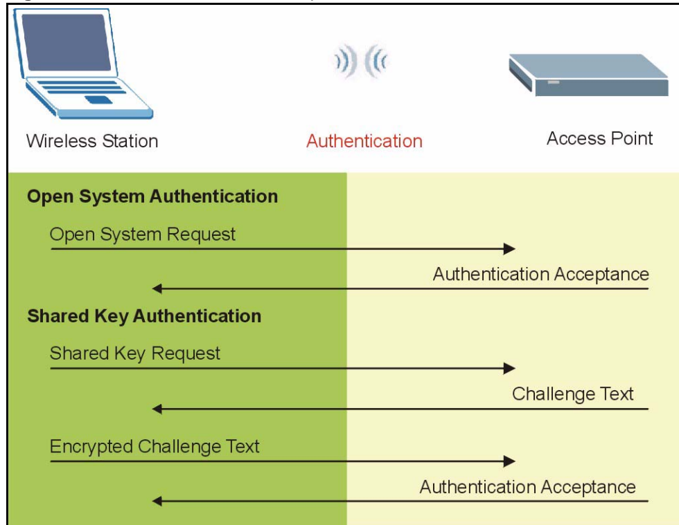
Figure 487 WEP Authentication Steps
