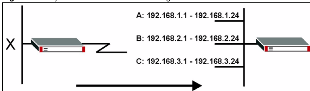
Figure 54 Physical Network & Partitioned Logical Networks
