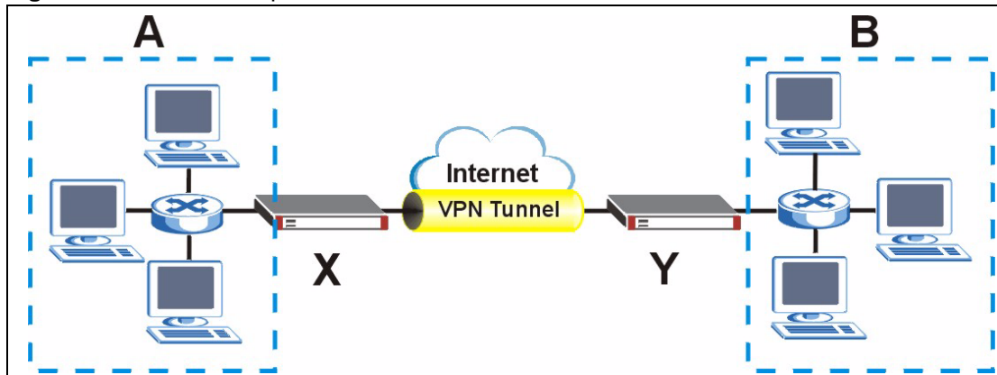
Figure 168 VPN: Example
