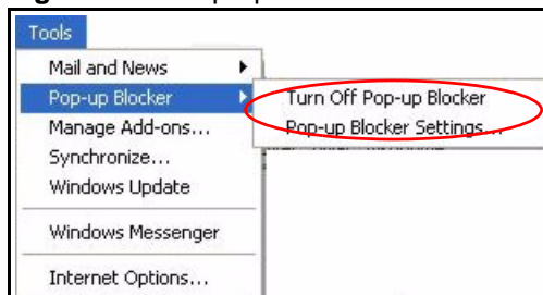
Figure 445 Pop-up Blocker
