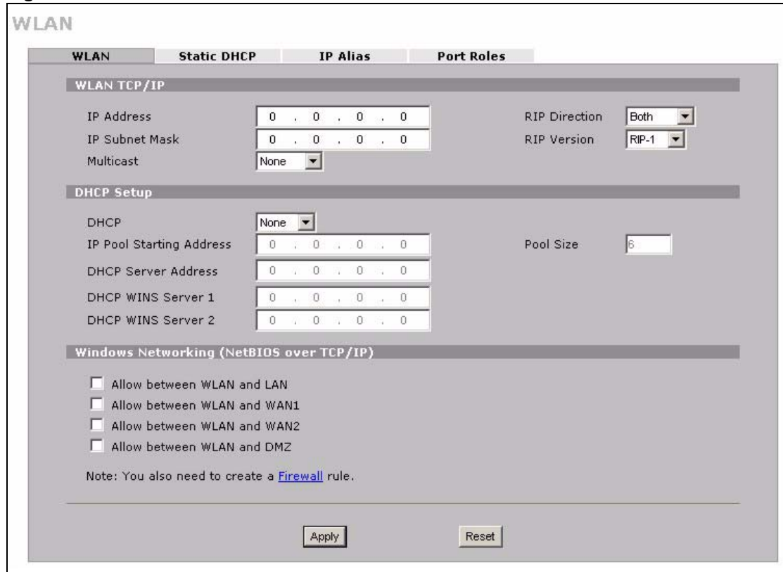
Figure 84 NETWORK > WLAN
