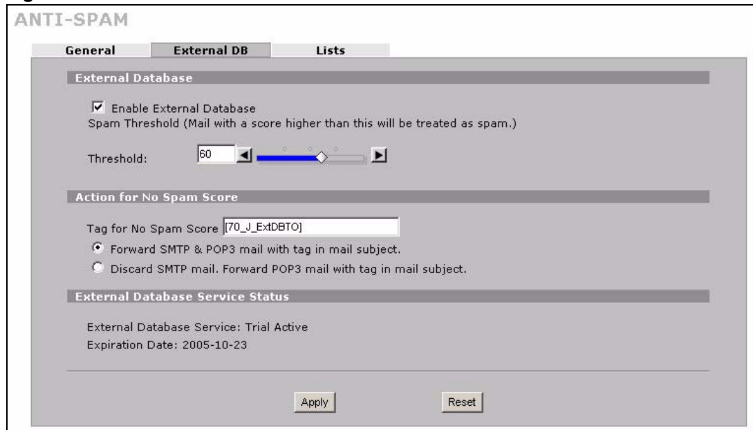
Figure 151 SECURITY > ANTI-SPAM > External DB
