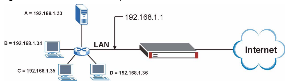
Figure 366 Server Behind NAT Example
