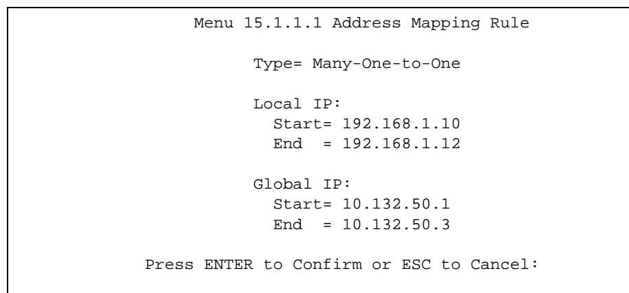
Figure 377 Example 4: Menu 15.1.1.1: Address Mapping Rule
