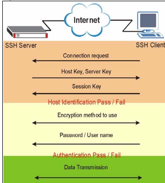
Figure 250 How SSH Works
