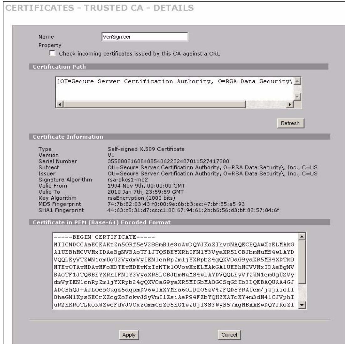
Figure 201 SECURITY > CERTIFICATES > Trusted CAs > Details
