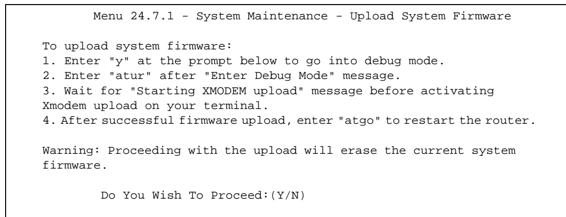
Figure 423 Menu 24.7.1 As Seen Using the Console Port
