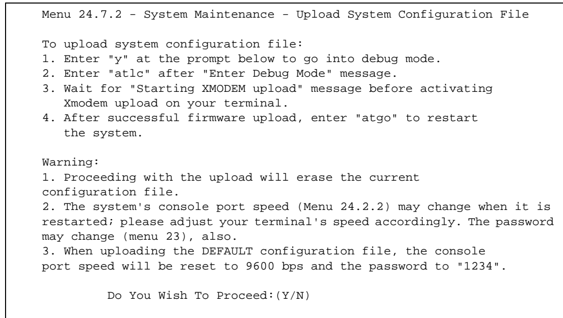
Figure 425 Menu 24.7.2 As Seen Using the Console Port
