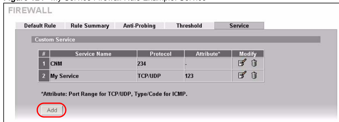
Figure 124 My Service Firewall Rule Example: Service
