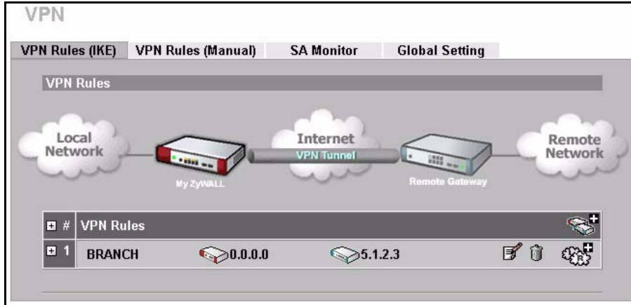
Figure 500 Branch Office VPN Rule
