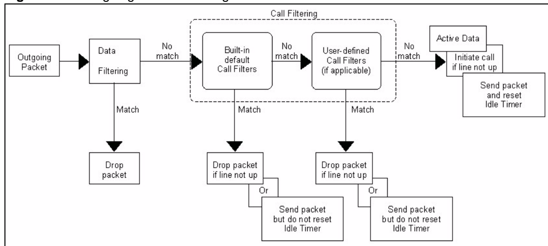
Figure 382 Outgoing Packet Filtering Process
