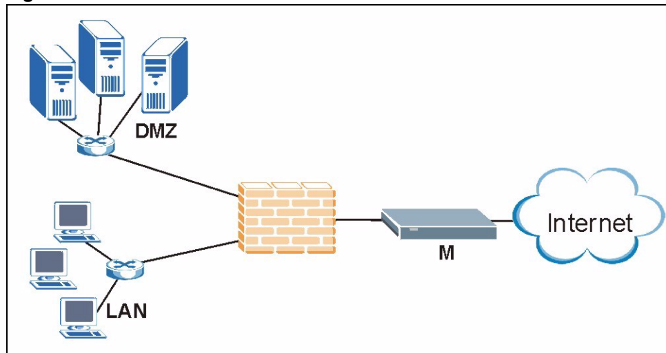
Figure 130 Network Intrusions
