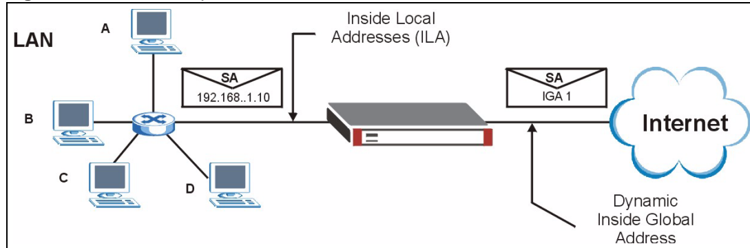
Figure 367 NAT Example 1
