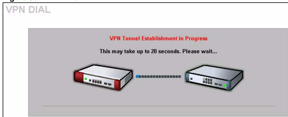
Figure 504 VPN Dial
