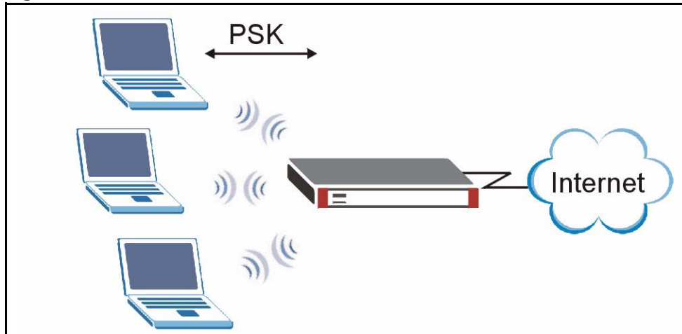
Figure 92 WPA-PSK Authentication
