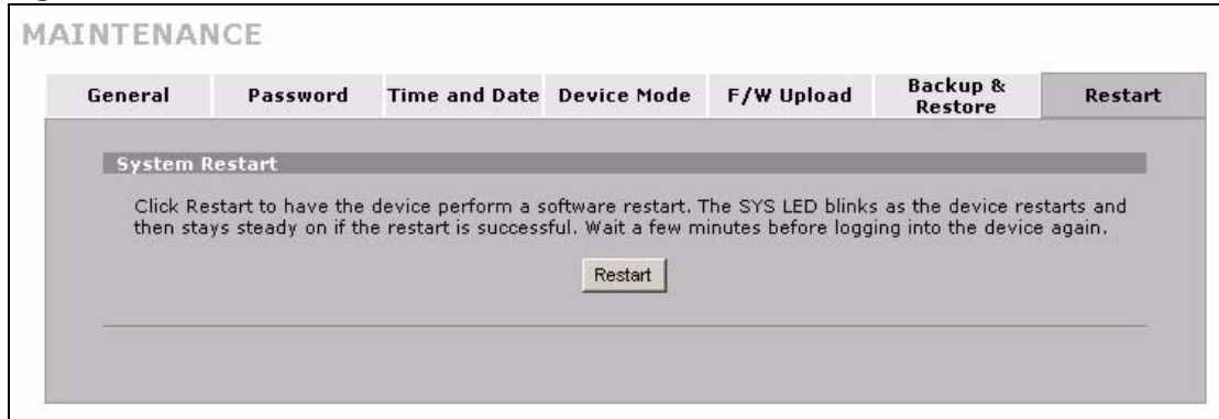
Figure 304 MAINTENANCE > Restart
