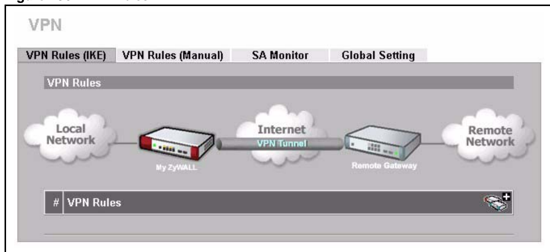
Figure 496 VPN Rules
