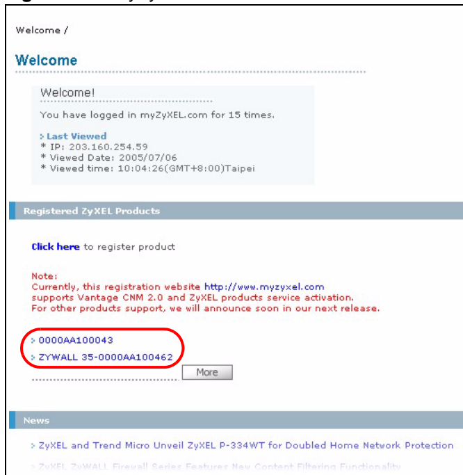
Figure 160 myZyXEL.com: Welcome
