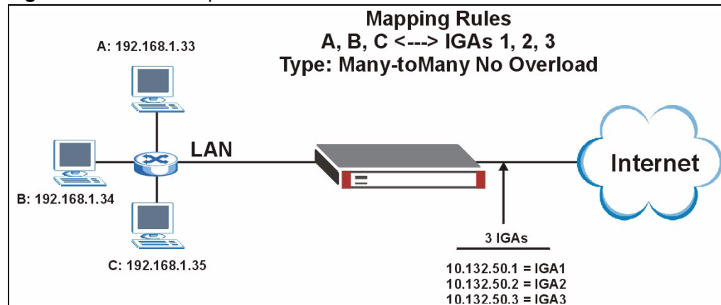
Figure 376 NAT Example 4
