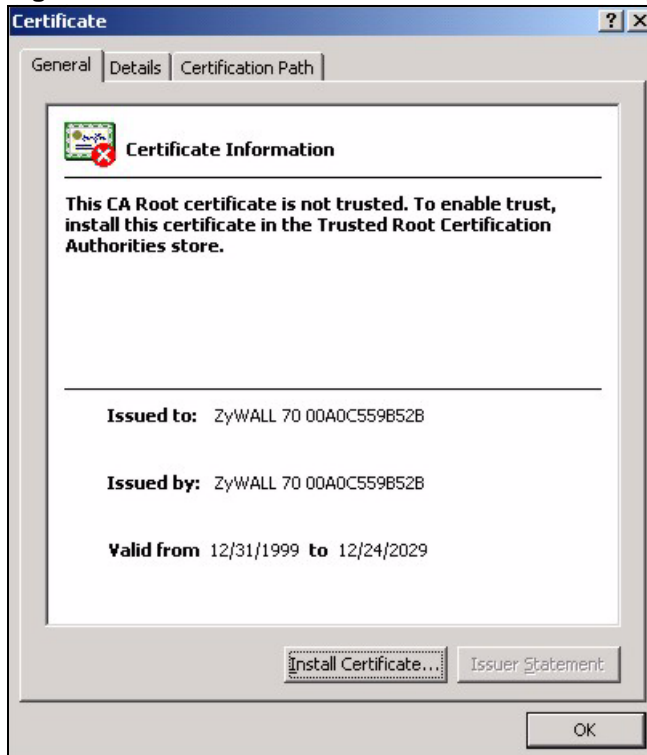
Figure 510 Certificate General Information before Import
