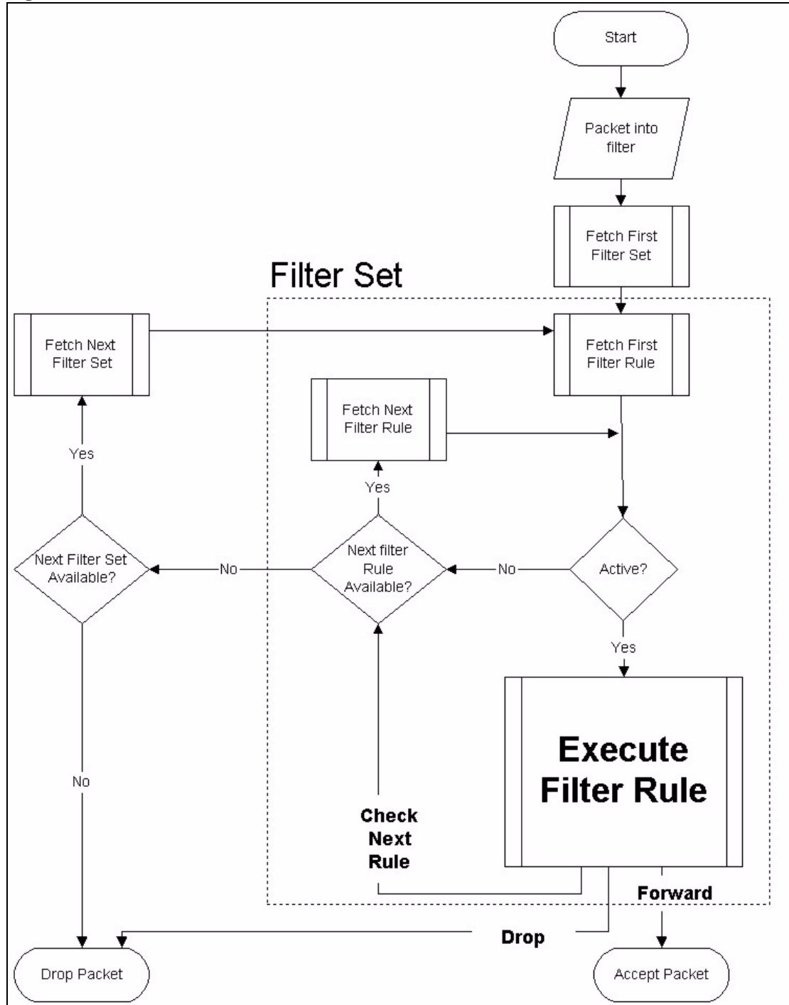
Figure 383 Filter Rule Process
