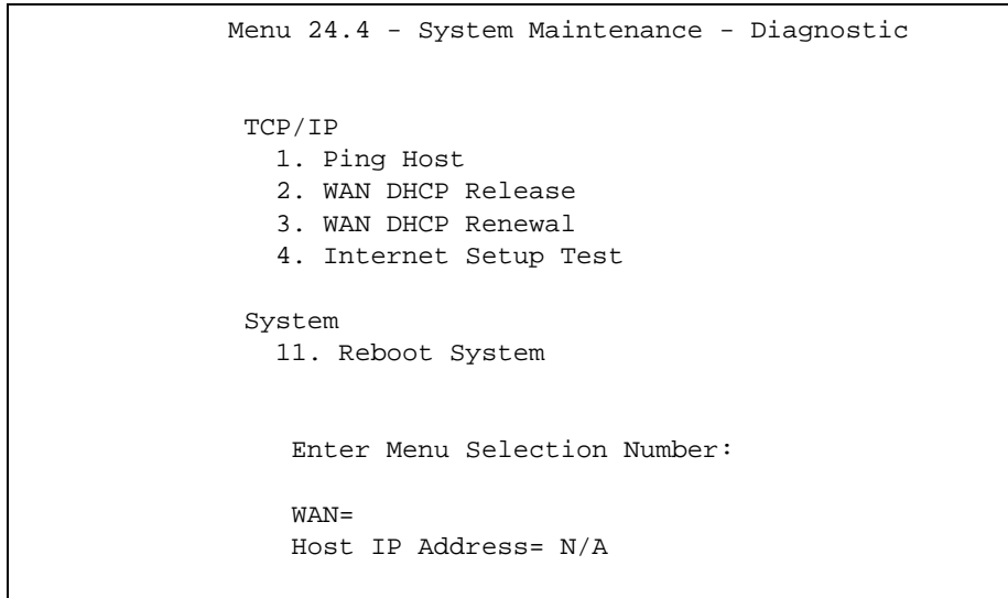
Figure 406 Menu 24.4: System Maintenance: Diagnostic
